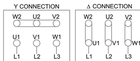
Figure 1: Connection types Y/D
